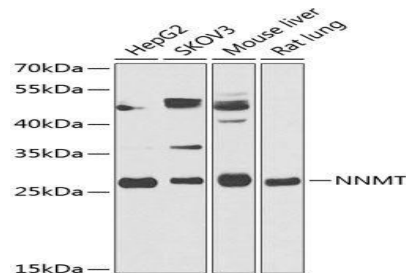
WesternBlot (WB) analysis of NNMT polyclonal antibody
